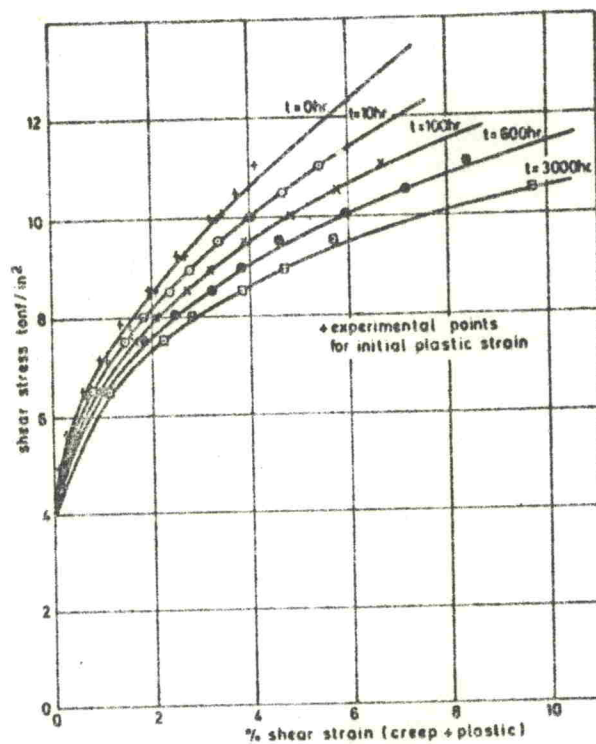
FIG. 9 TYPICAL ISOCHRONOUS CURVES DRAWN FROM TORSION CREEP RESULTS (0.18 PERCENT CARBON STEEL AT 400^{\circ}\text{C} )
