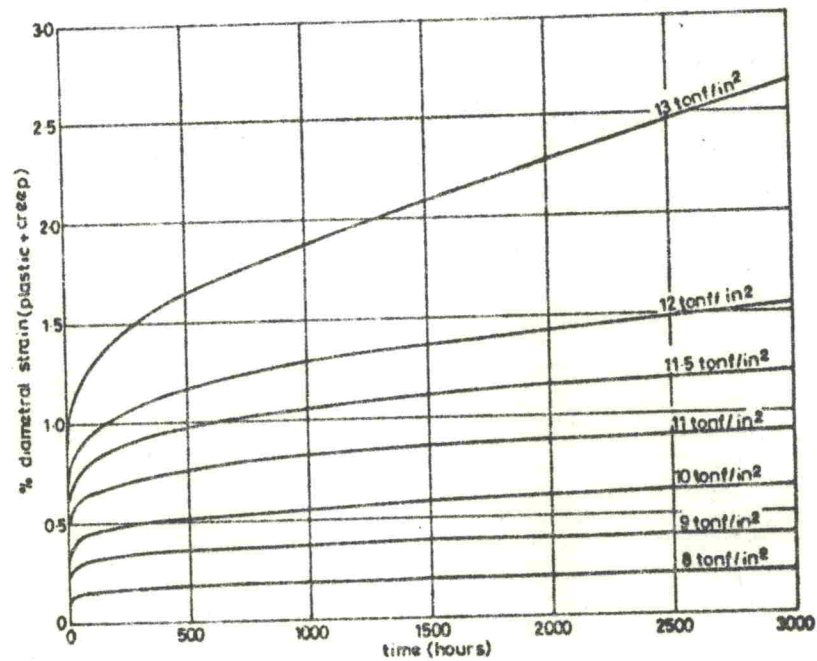
FIG. 8 EXPERIMENTAL PRESSURE CREEP CURVES FOR CYLINDERS ( K=2 ) (0.18 PERCENT CARBON STEEL AT 400^{\circ}\text{C} )
